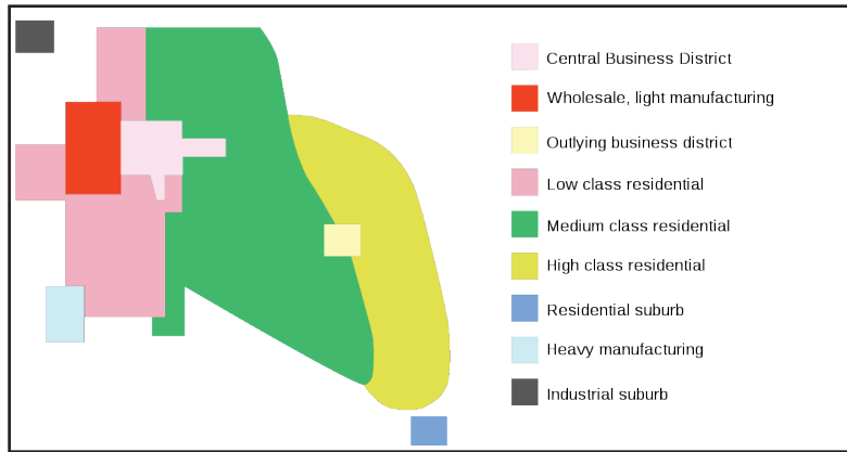
Figure 12.21 | Multiple-Nuclei Theory
